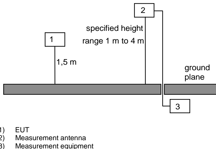
Figure B.4: Measurement arrangement No.1
