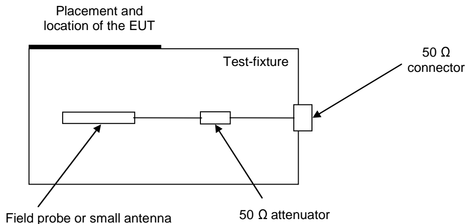
Figure C.1: Test fixture
